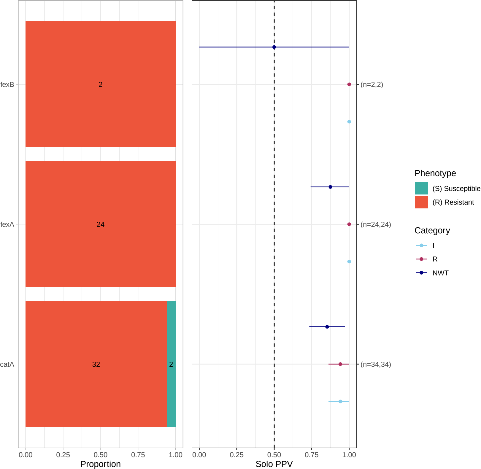
Solo markers for class: PHENICOL vs phenotype for drug: CHL
